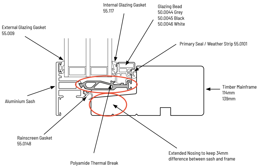
VELFAC 200 ENERGY key system components
