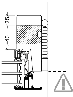
VELFAC 200 ENERGY
