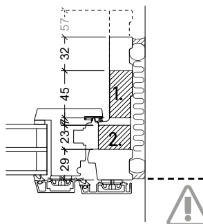
VELFAC In, 149mm + 174mm frame 1. + 2. ⇒ see text
