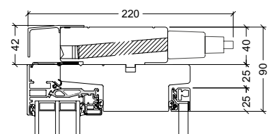
Installed on 3 + 1 window solution
