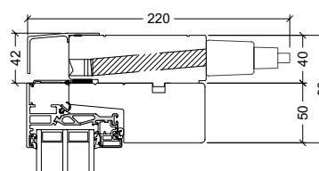
Installed on 114mm mainframe
