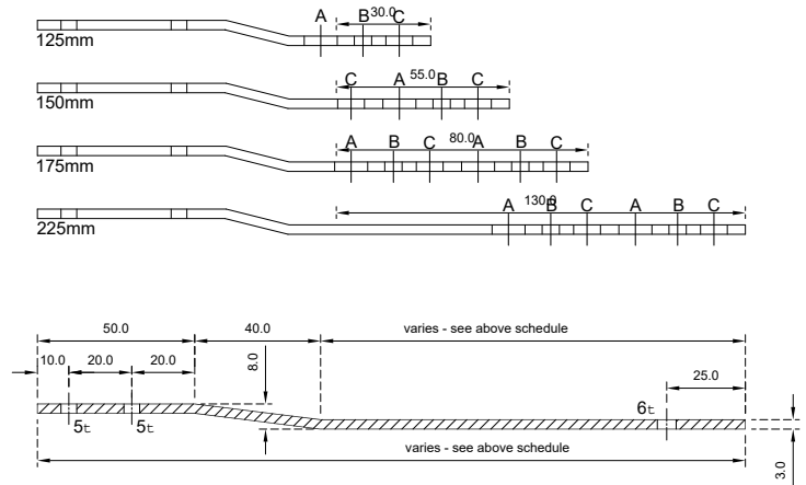
Section - staggered fixing
