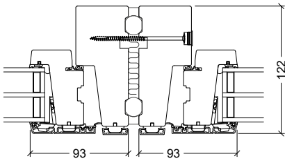
Horizontal coupling Window to window
