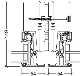
T Section Coupling
