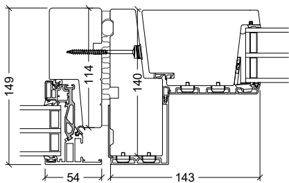
with VELFAC Ribo inward opening door (cover profile*)
