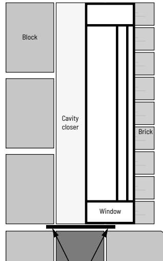
Bridging plate to span from out to in
