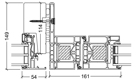
with VELFAC Aluminium door, outward and inward opening (5mm x 50mm screw)
