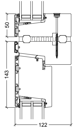
Vertical coupling Door with fixed top-light
