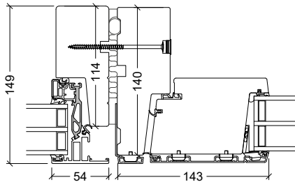
with VELFAC Ribo outward opening door (cover profile*)
