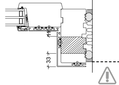
VELFAC Ribo sliding door opening part, jamb
