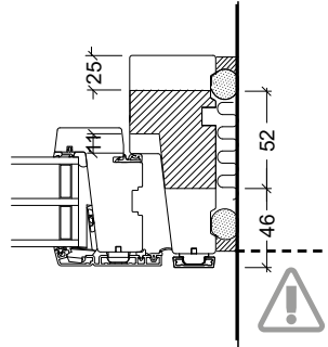
VELFAC Ribo outward opening windows and doors
