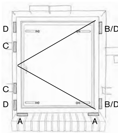
Sidehinged VELFAC 200
