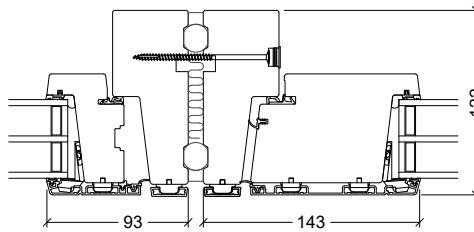
Vertical coupling Window to outward opening door
