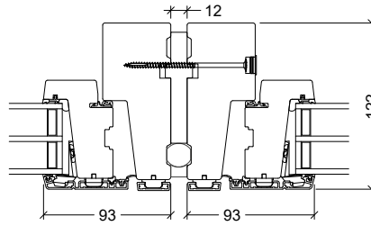
T Section coupling Window to window
