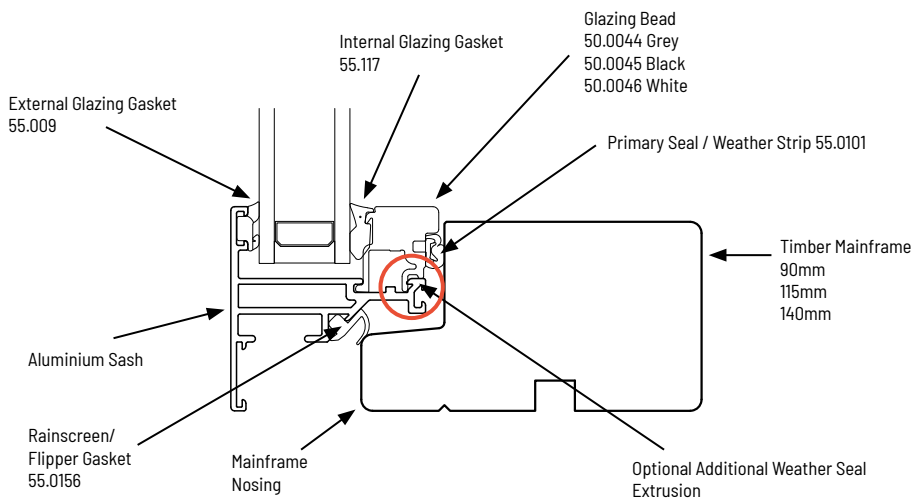
VELFAC 200 key system components
