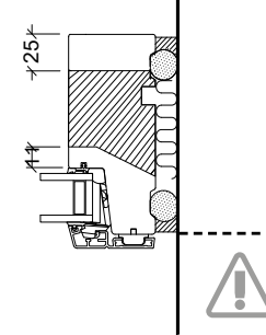
VELFAC Ribo fixed frame, 2-layer glazing
