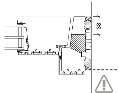
VELFAC Ribo inward opening doors
