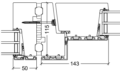
Horizontal coupling Window to inward opening door
