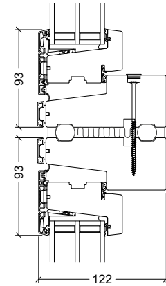
Vertical coupling Window to window
